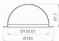
SMT-062H 6.2-inch Dome Cover
