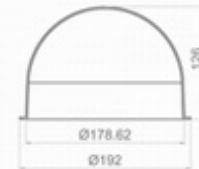
SMT-070H126-PC 7.0-inch Vandal-proof Dome Cover
